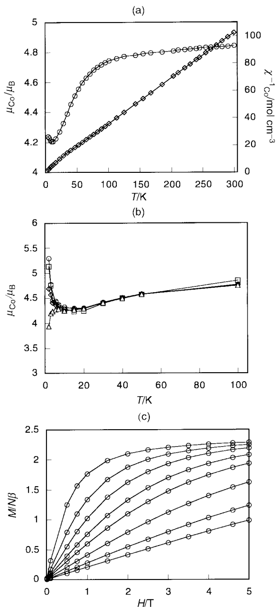
Fig. 8 (a) Plots of \mu_{\text{Co}} (○) and \chi^{-1}_{\text{Co}} (□) vs. temperature for Co(tcm) 2 in a field of 1 T. (b) \mu_{\text{Co}} values observed in fields of 10 000 (△), 5000 (◇), 1000 (□) and 100 (○) Oe, over the range 2–100 K. (c) High field magnetisation isotherms obtained at temperatures of 2 (top), 3, 4, 5.5, 7, 10, 15 and 20 K (bottom). The solid lines are a guide to the eye.
