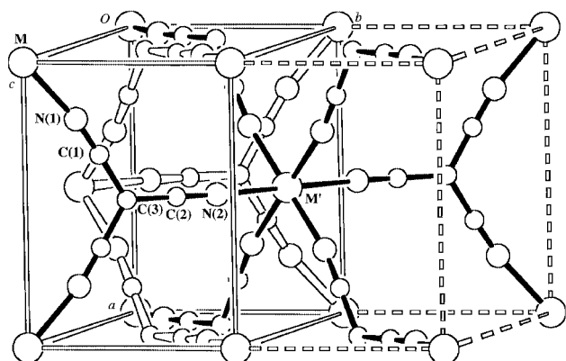
Fig. 2 The unit cell and numbering scheme for M(tcm)_2 . One framework is continued into an adjoining cell to illustrate the rutile relationship.
