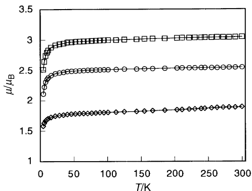
Fig. 11 Plots of \mu vs. temperature for \text{Ni}(\text{tcm})_2 (□), \text{Ni}/\text{Cu}(\text{tcm})_2 (50:50) (○) and \text{Cu}(\text{tcm})_2 (◇) in a field of 1 T. The solid lines are a guide to the eye.
