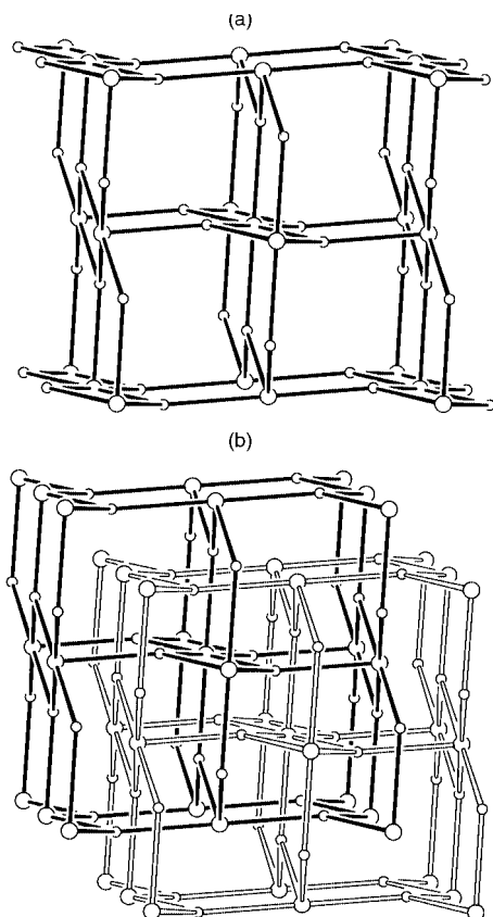
Fig. 1 (a) A single rutile-like framework in M(tcm)_2 . Only the metal atoms and central carbon atoms of the tcm^- anion are shown. The bonds represent C–C≡N–M linkages. (b) Two interpenetrating frameworks.
