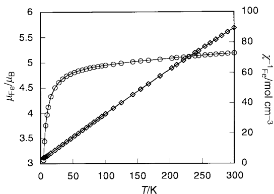
Fig. 7 Plots of \mu_{\text{Fe}} (○) and \chi^{-1}_{\text{Fe}} (□) vs. temperature for Fe(tcm) 2 in a field of 1 T. The solid lines are a guide to the eye.
